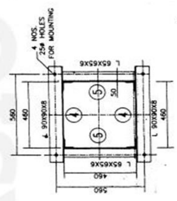
132 KV 1PH CT STRUCTURE ( JBIC ) ABC/132/DWG/CT3/LOT-IV
