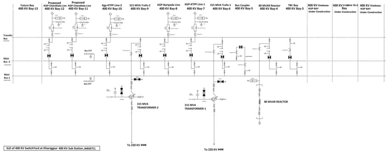
SLD of 400 KV SwitchYard at Kharagpur- 400 KV Sub Station ,WBSETCL
