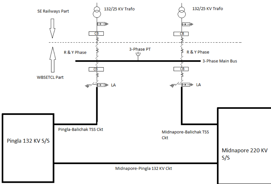
Single Line Diagram of BALICHAK TSS
