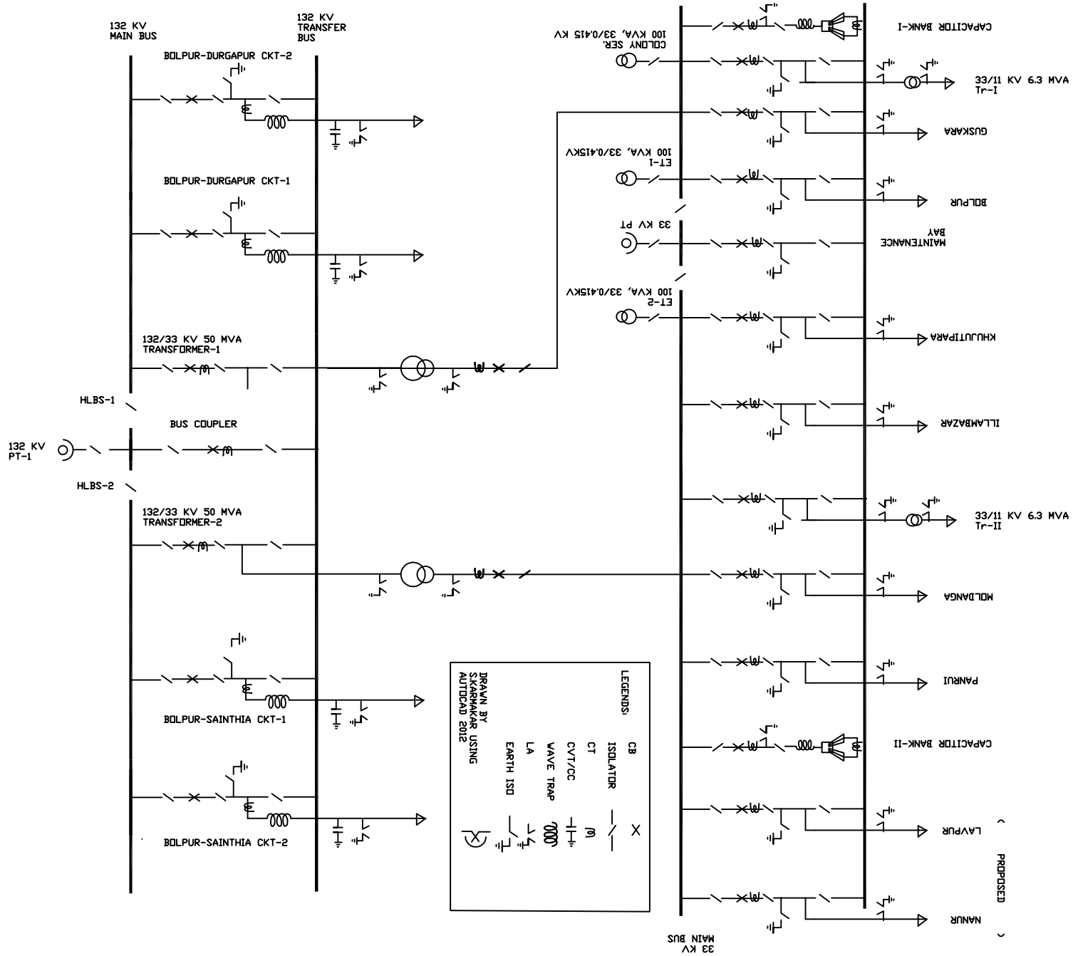
SINGLE LINE DIAGRAM OF BOLPUR 132/33 KV SUB-STATION
