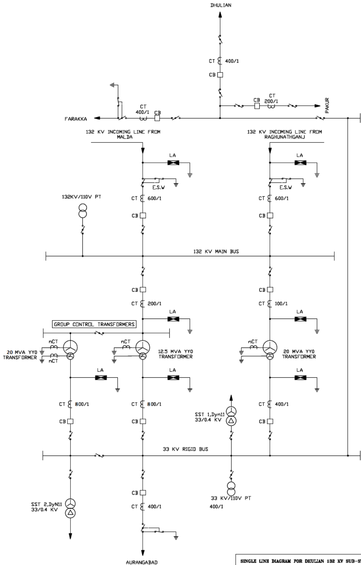
SINGLE LINE DIAGRAM FOR DEHULIAN 132 KV SUB-STATION
