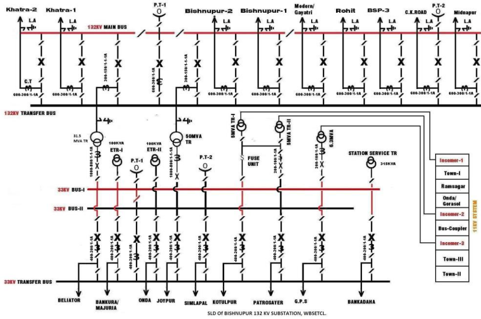
SLD OF BISHNUPUR 132 KV SUBSTATION, WBSSETCL.
